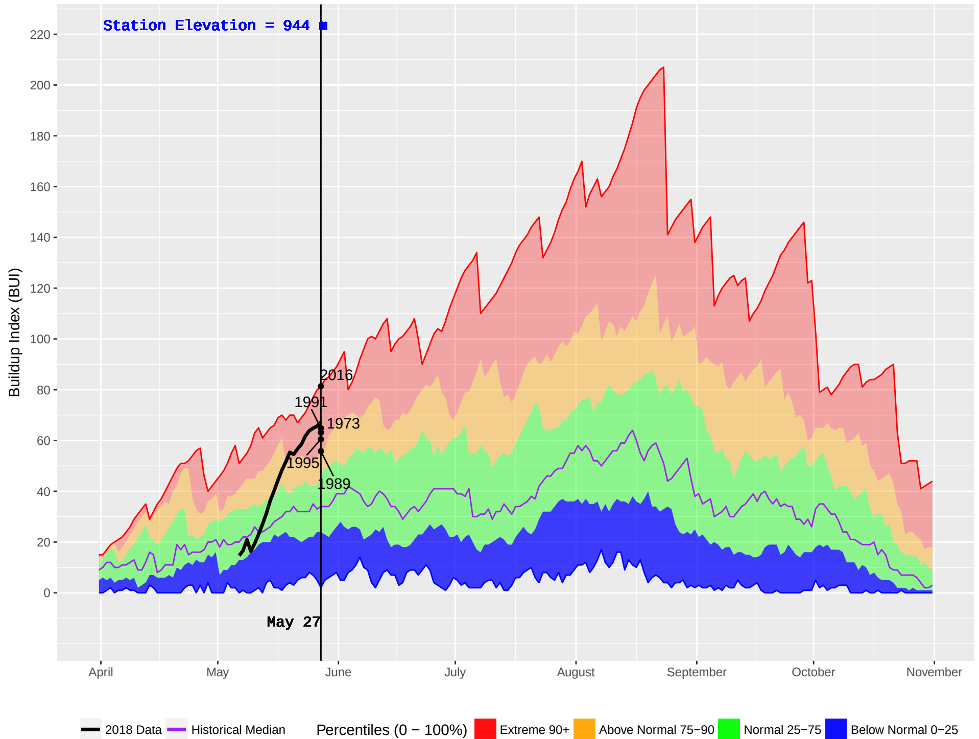
GRASSY PLAINS HUB (161) : Historical (1970–2016) and Current (2018) Noon Buildup Index (BUI)
