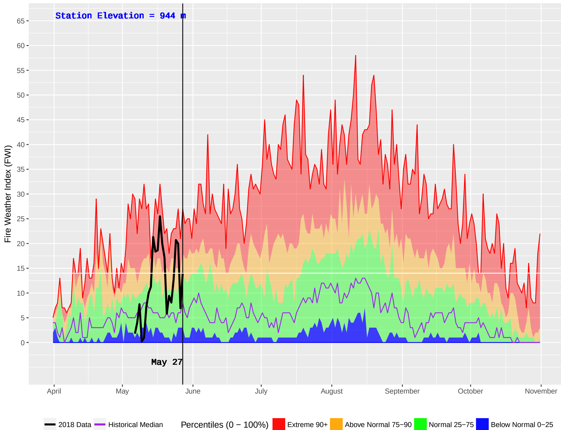
GRASSY PLAINS HUB (161) : Historical (1970–2016) and Current (2018) Noon Fire Weather Index (FWI)
