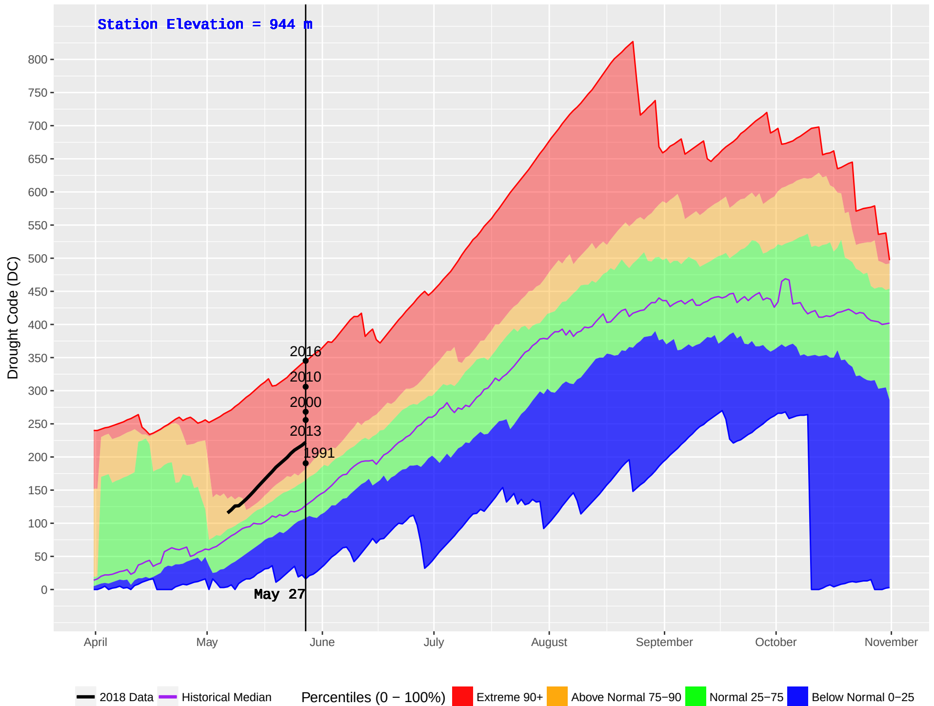
GRASSY PLAINS HUB (161) : Historical (1970–2016) and Current (2018) Noon Drought Code (DC)
