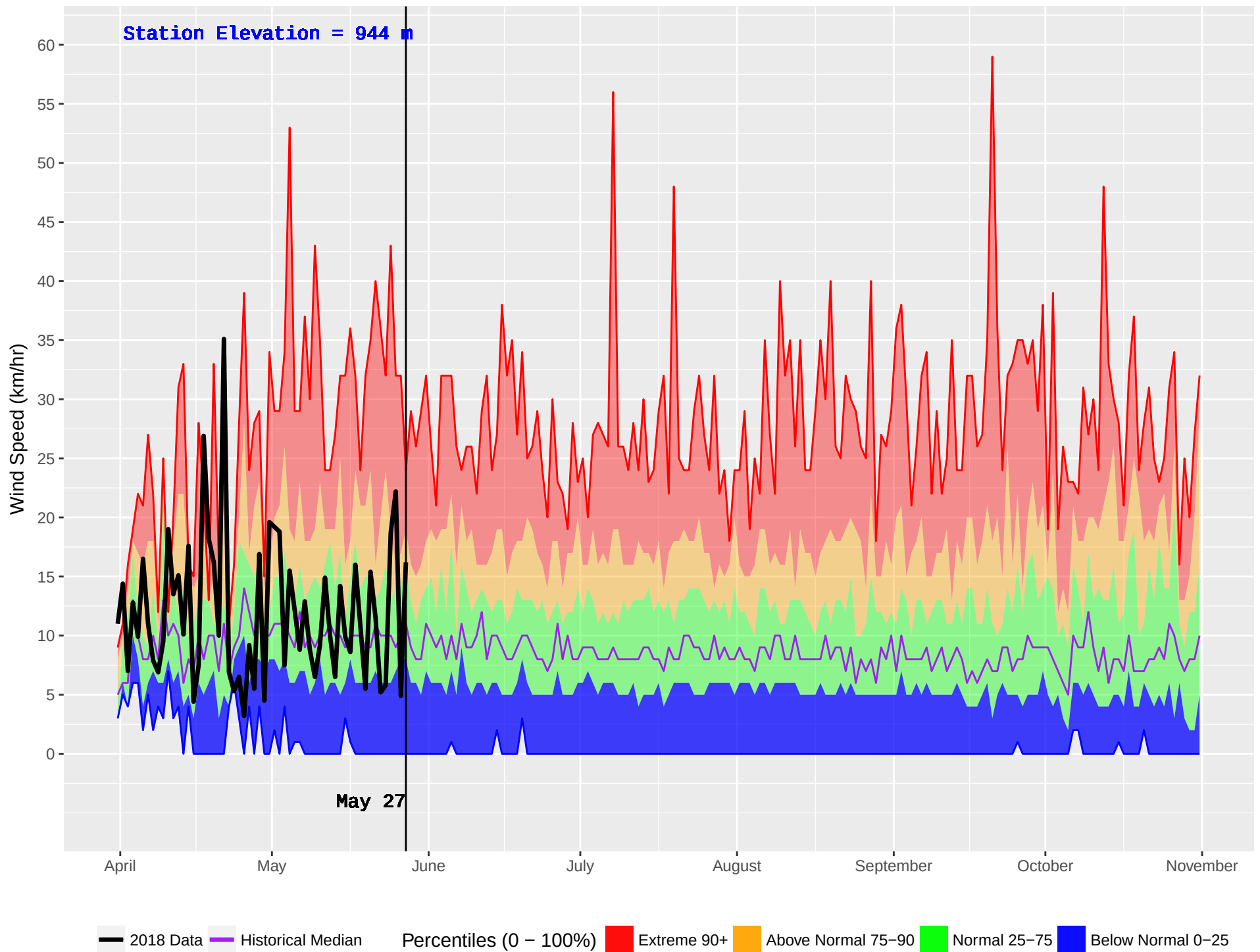
GRASSY PLAINS HUB (161) : Historical (1970–2016) and Current (2018) Noon Wind Speed
